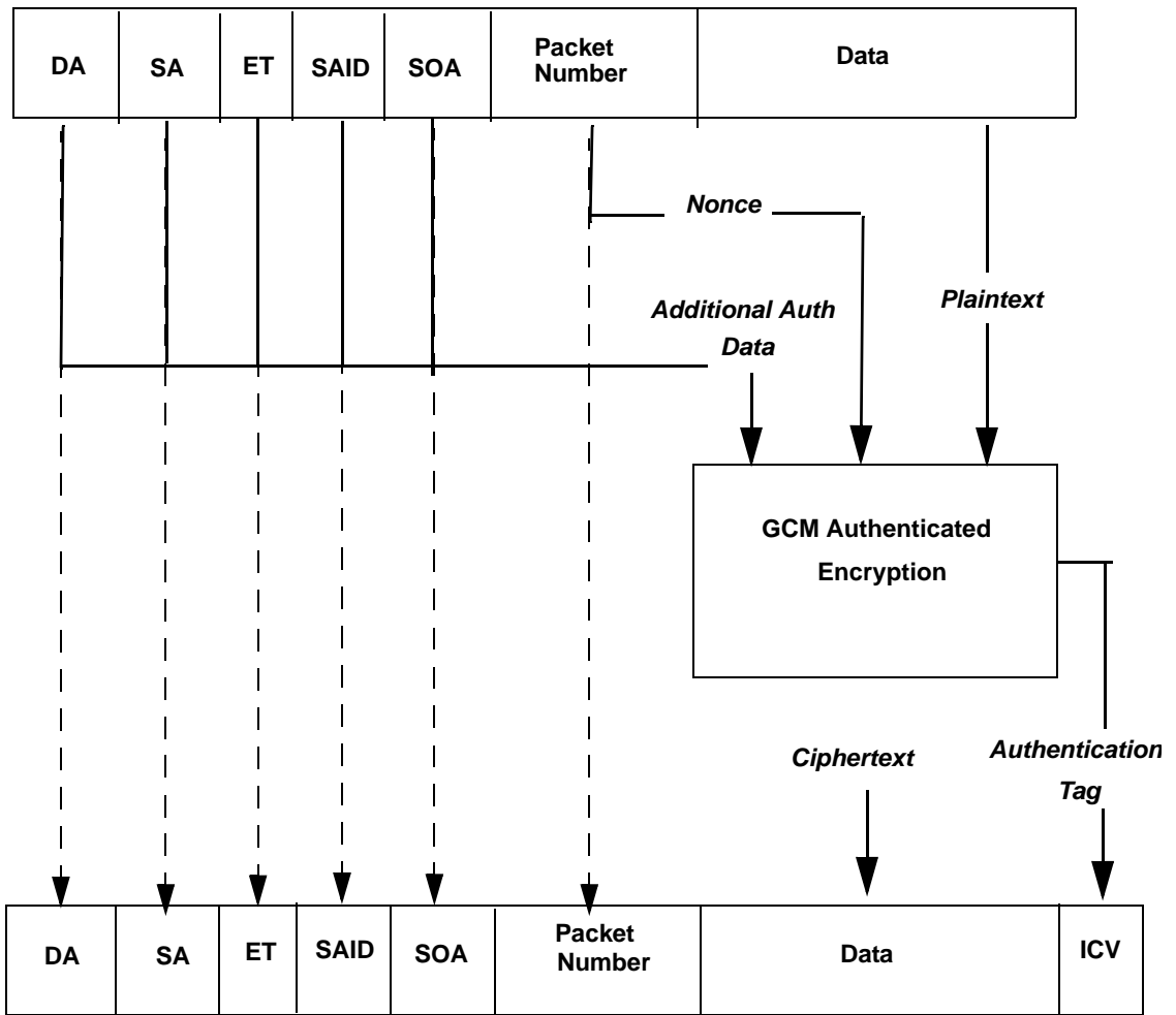
FIGURE: Using MACsec with GCM
