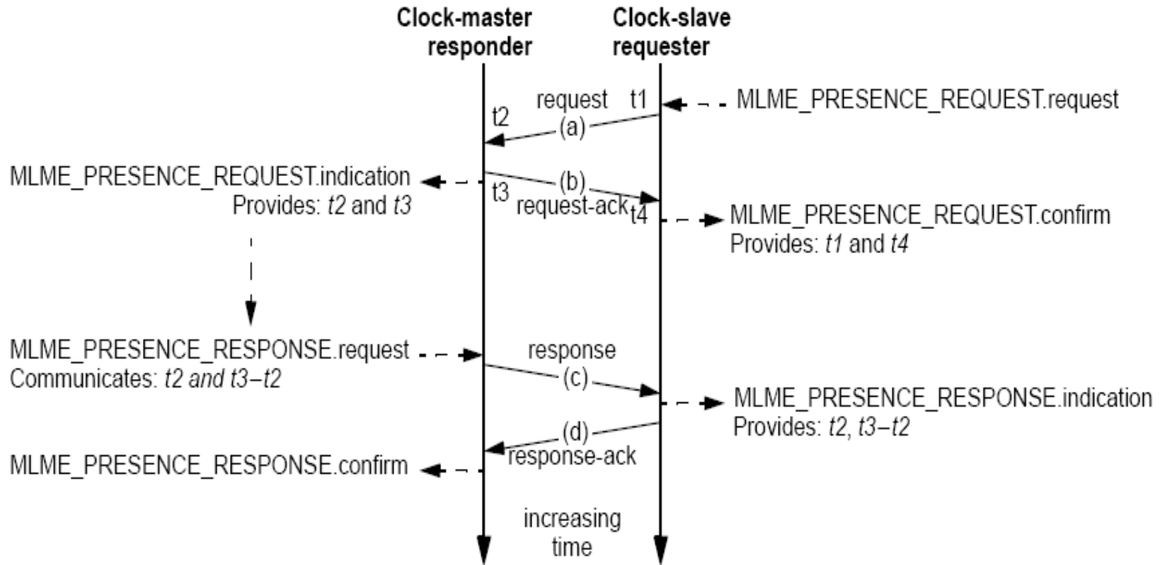
Figure 12.2—802.11v time-synchronization interfaces
