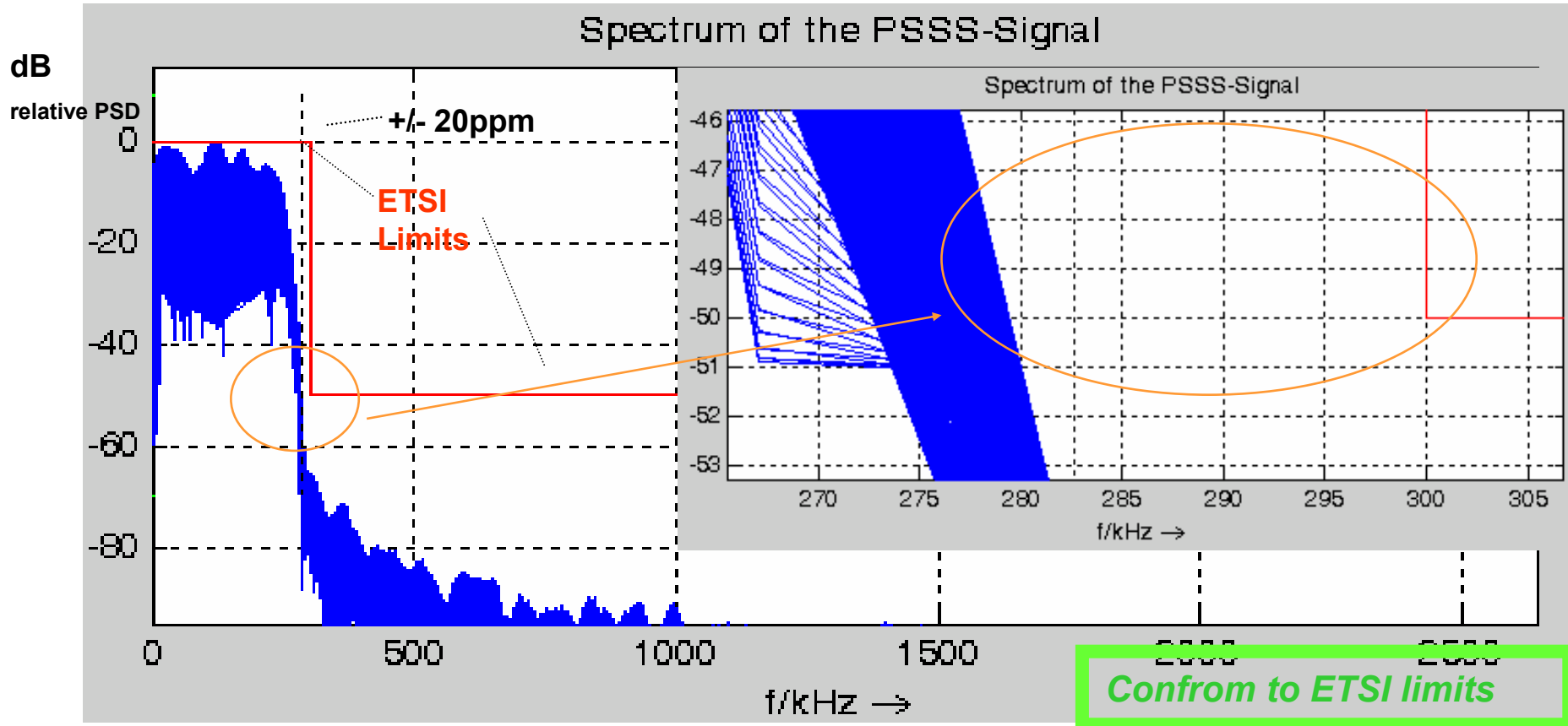
Simulations of the relative PSD in dB for the PSSS signal at 480 kchips/s, 225 kbit/s, +/- 20ppm. Conditions: non linear, precoding
