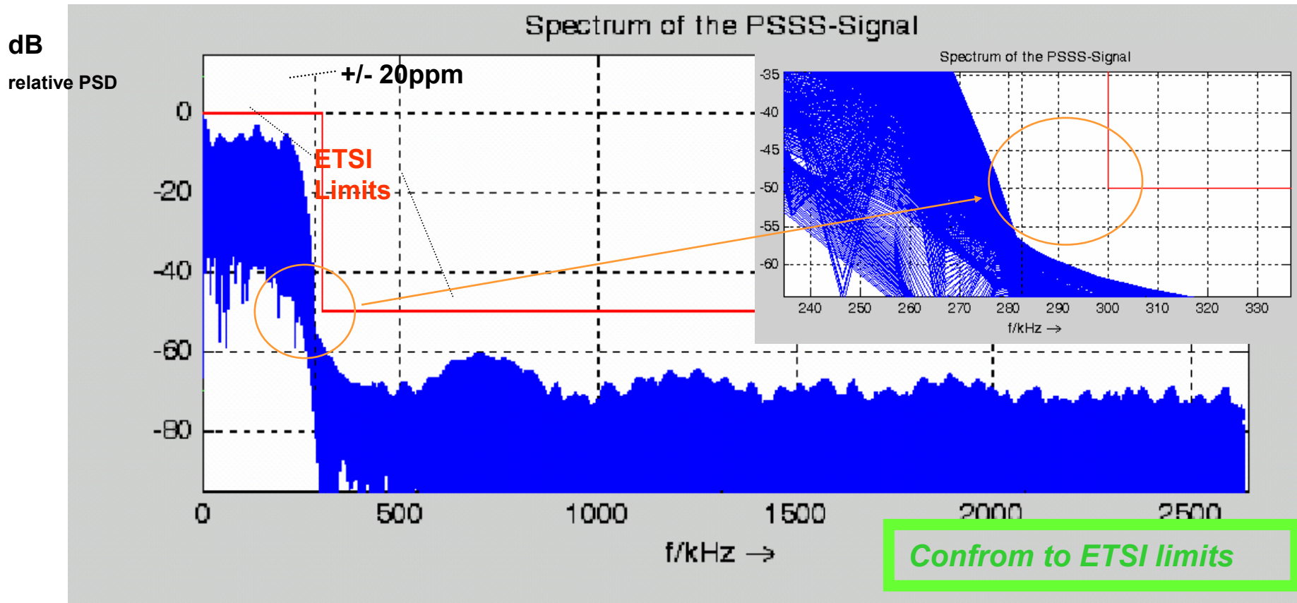
Simulations of the relative PSD in dB for the PSSS signal at 480 kchip/s, 225 kbit/s, +/-20 ppm
