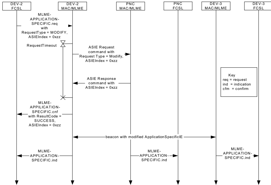
Figure 147b—Message sequence chart for a DEV modifying an ASIE in the beacon.
