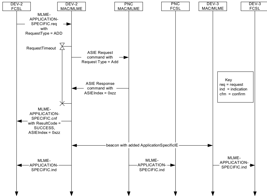
Figure 147a—Message sequence chart for a DEV adding an ASIE to the beacon.
