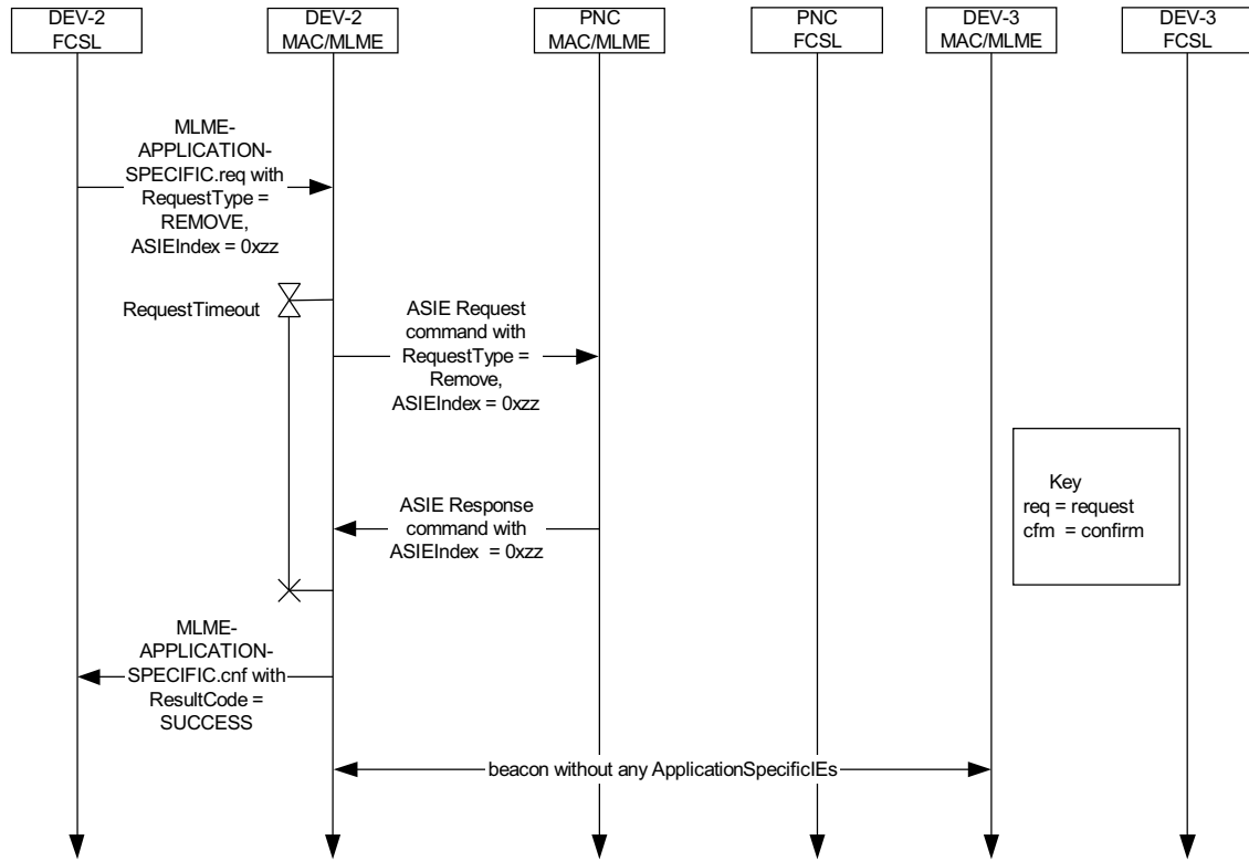
Figure 147c—Message sequence chart for a DEV removing an ASIE from a beacons
