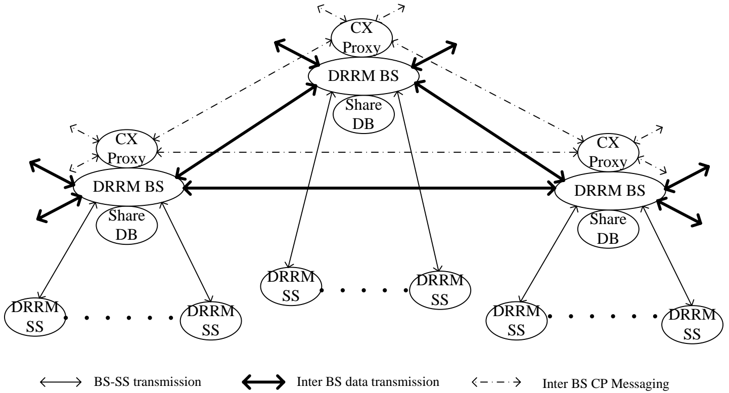
Figure h18a – System Architecture within unconvertant systems
