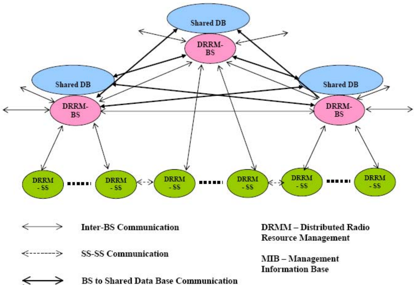
Figureh18 –System Architecture within conversant systems
