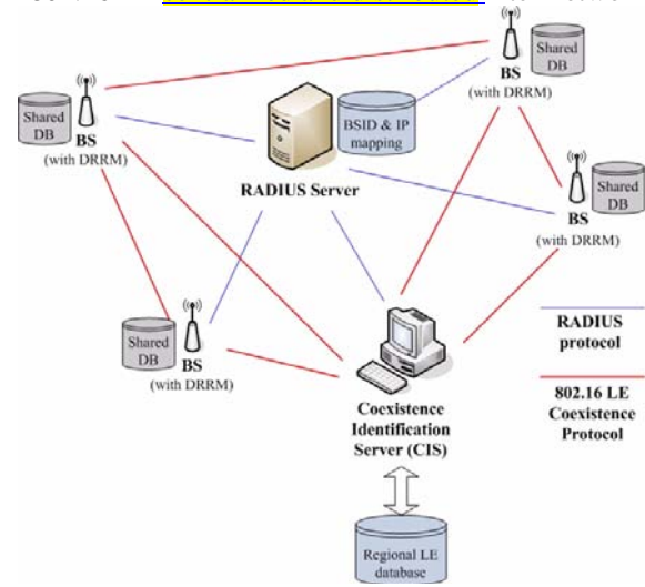
Figure h19 – centralized network architecture
