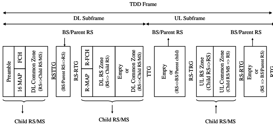
Figure 4 RS frame structure
