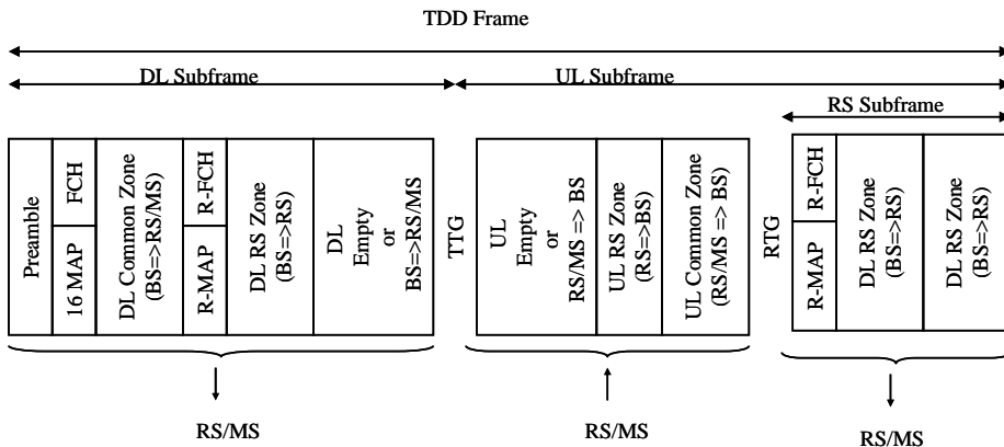
Figure XXX. MMRBS frame structure.
