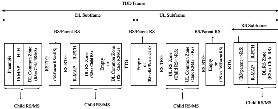
Figure XXX. Frame structure of RS with preamble transmission.
