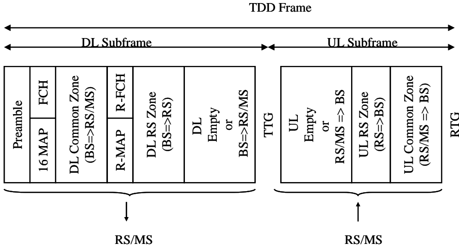
Figure 2 MMR-BS frame structure
