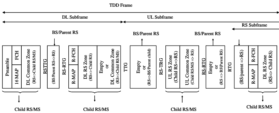
Figure 5 RS frame structure
