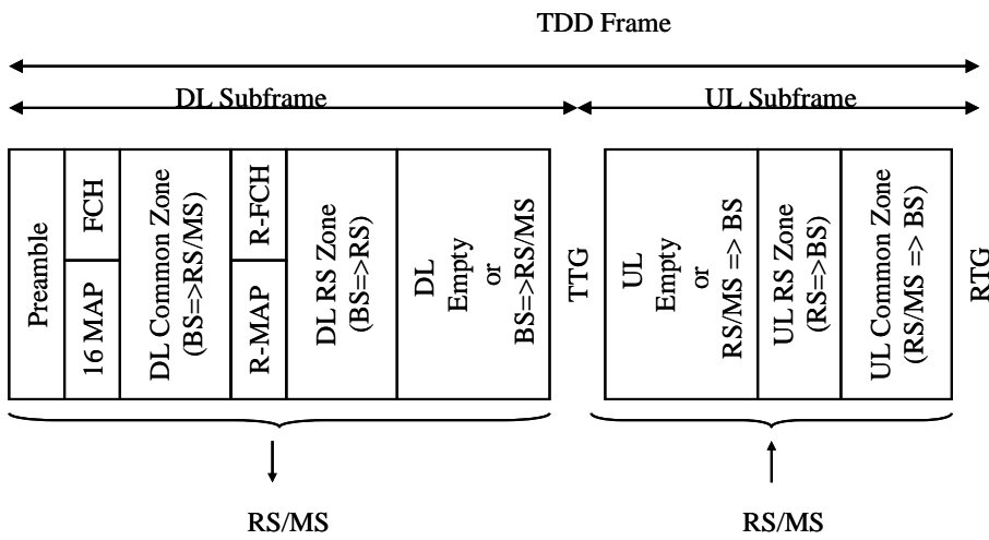
Figure 3 MMR-BS frame structure
