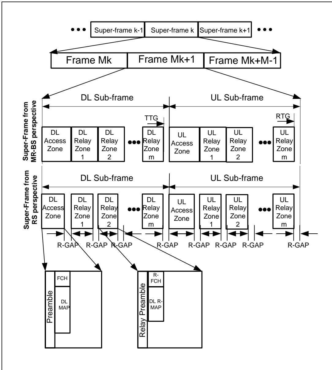
Figure yyy Example of an M frame MR-BS and RS k Super-Frames using relay preamble
