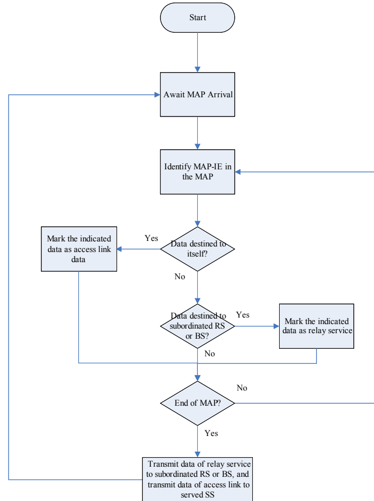
Figure xxx – Relay Service Flow Chart of RS
