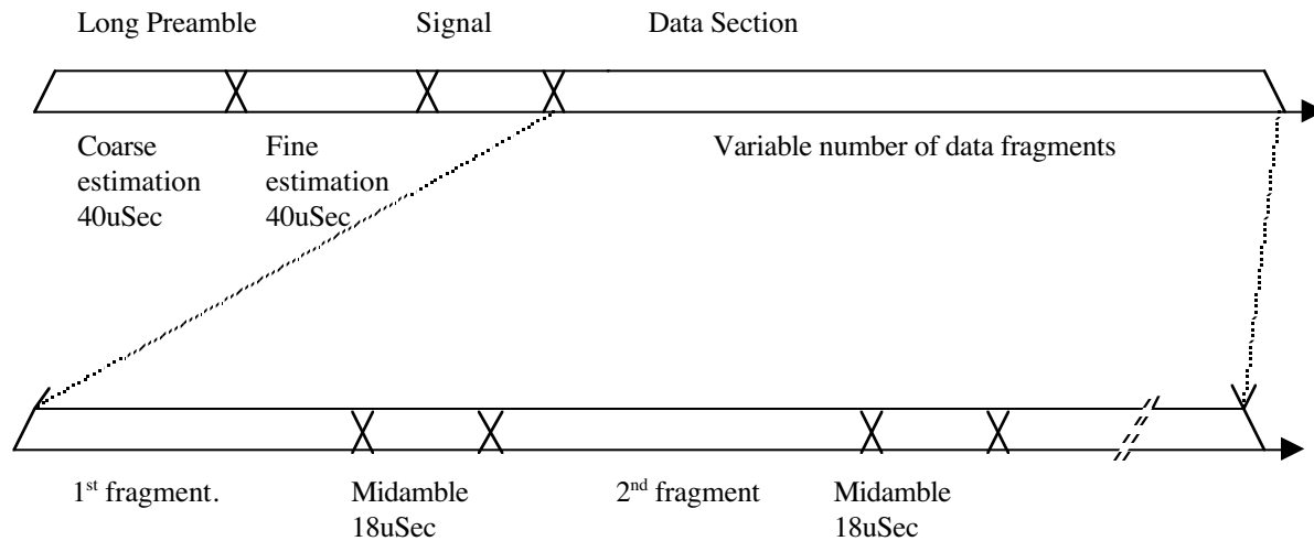
Figure 8 Structure of a packet with a long preamble and multiple data fragments with mid-ambles
