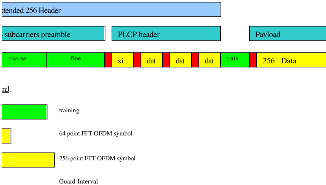
Figure 2 The FFT size switchover concept illustration
