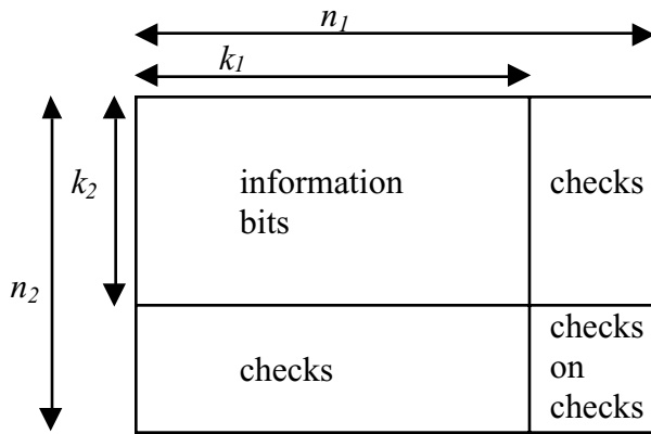
Figure 12 Figure 1 - Two-dimensional product code matrix
