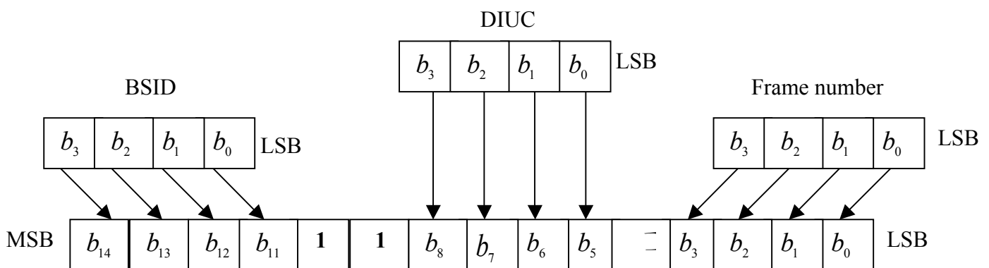
OFDM Scrambler Initialization Vector
