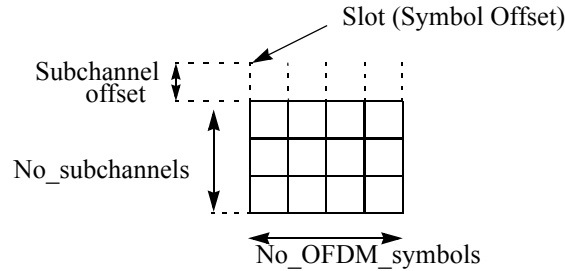
Figure 209—Example of the data region which defines the OFDMA allocation
