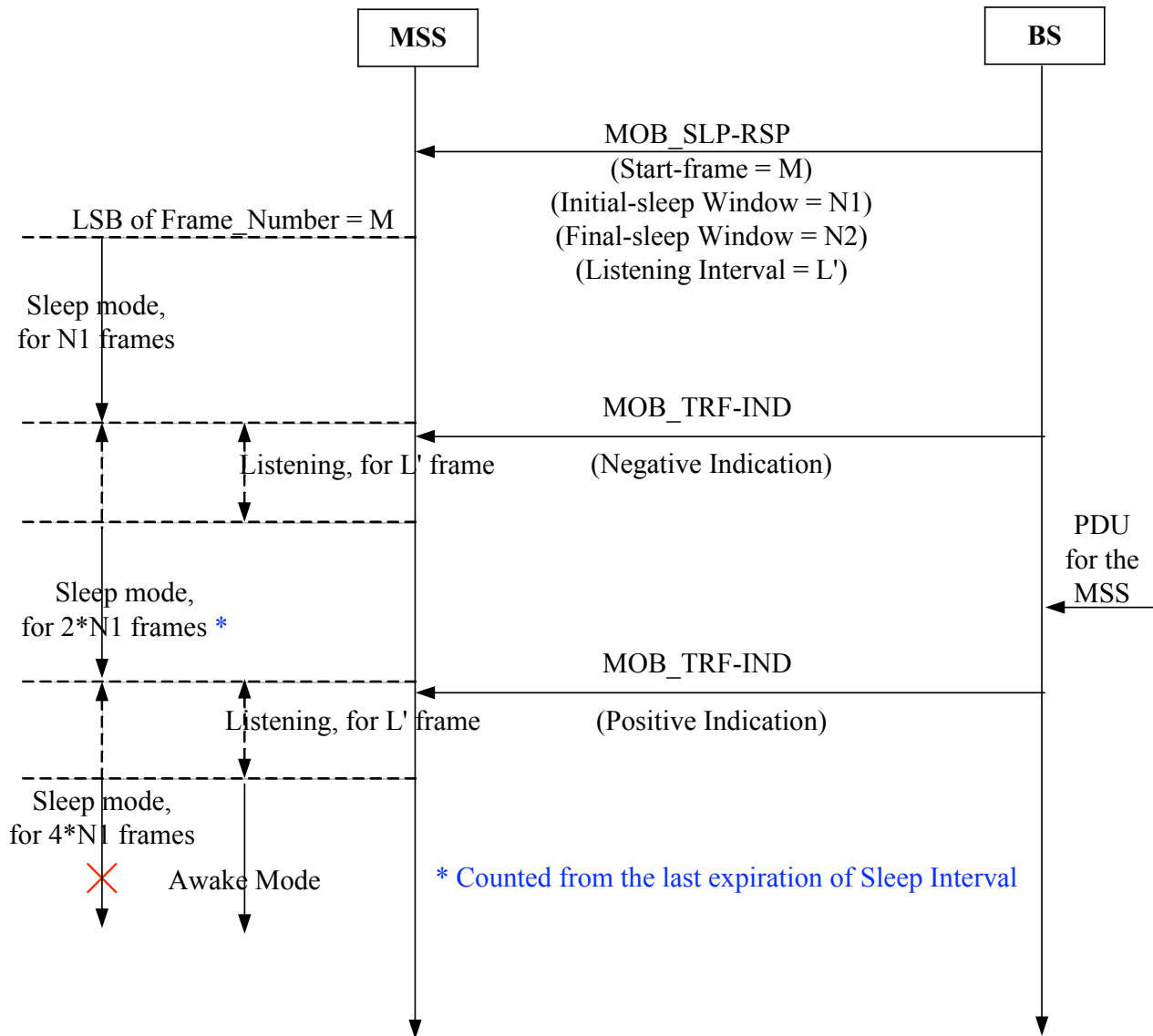
Figure D.12 – Sleep Mode – BS initiated
