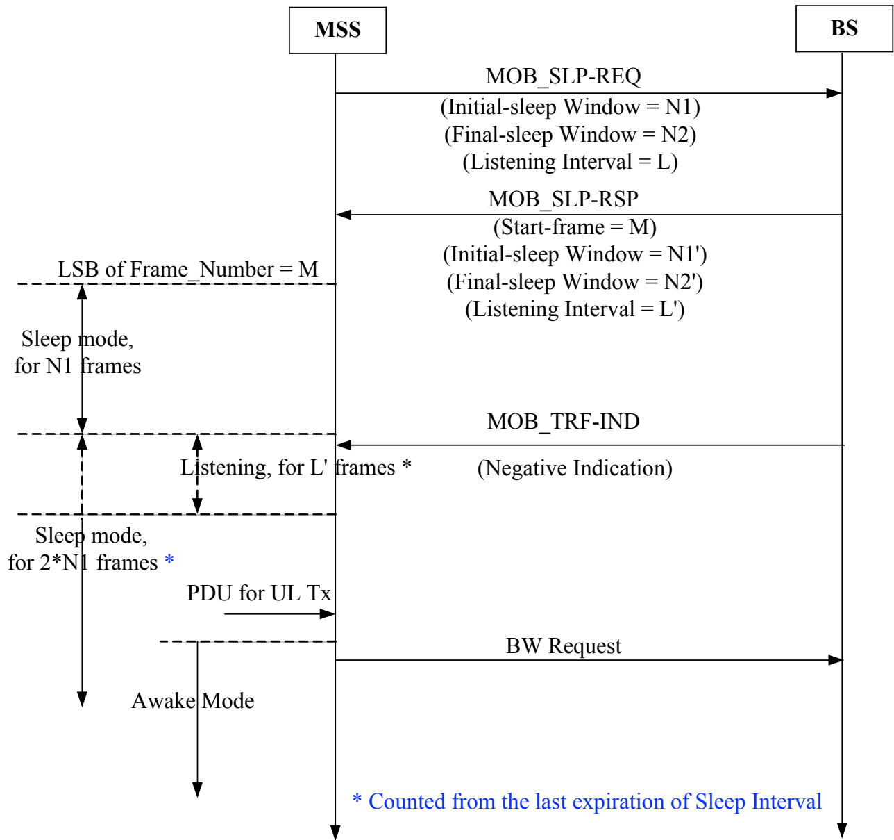
Figure D.13 – Sleep Mode – MSS initiated awakening
