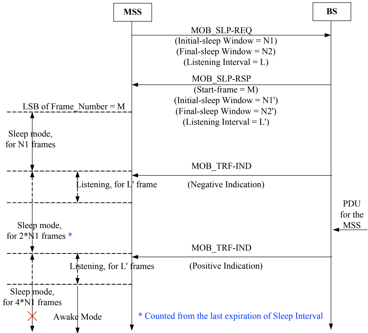
Figure D.11 – Sleep Mode – MSS initiated
