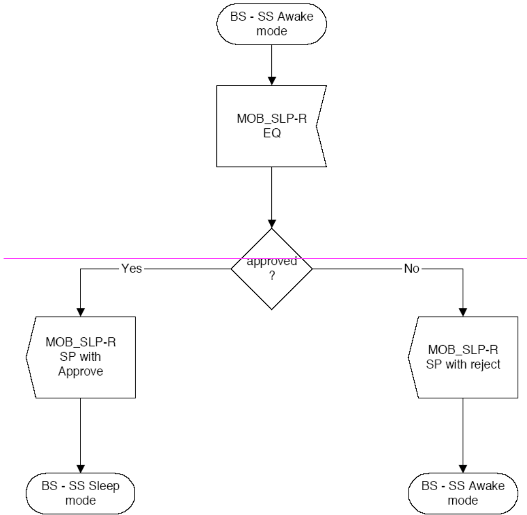
Figure 108m—BS-SS Awake Mode SDL Diagram
