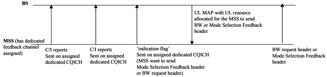
Fig. 1. Method for MSS to signal its intention for mode selection feedback or bandwidth request by using CQICH indication and Mode Selection Feedback MAC header
