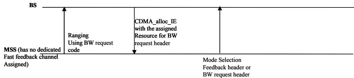
Fig. 2. Method for MSS to send mode selection feedback by using BW request ranging and Mode Selection Feedback MAC header.
