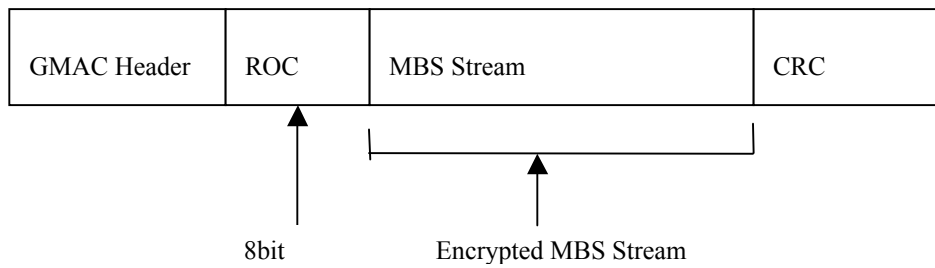
Figure 137a –MBS MAC PDU Ciphertext payload format
