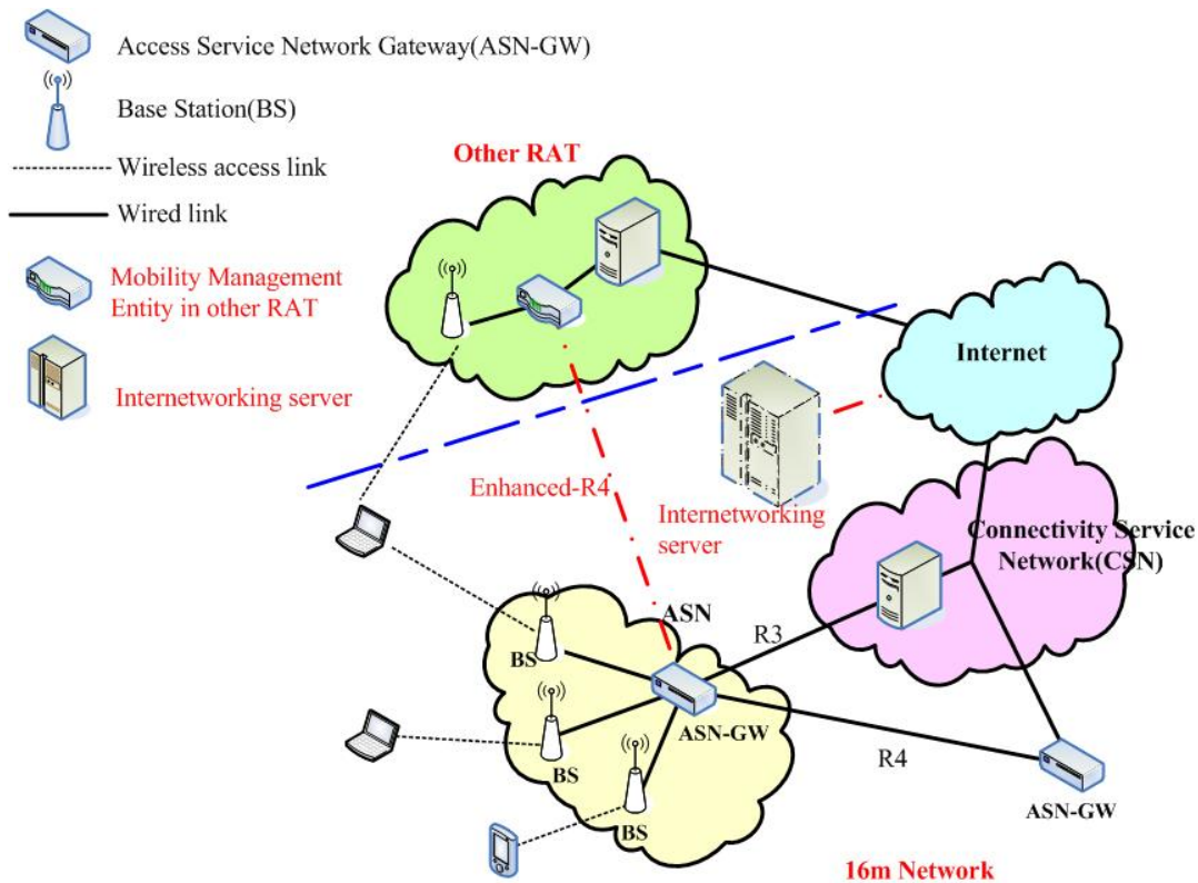
6 7 Figure 2. Inter-RAT Network architecture
