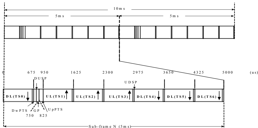
Figure 4: TD-SCDMA Radio frame structure
