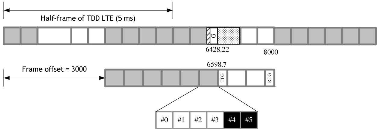
Figure 8 example of solution result when ratio of UL:DL = 1:3 for both IEEE 802.16m and TDD LTE
