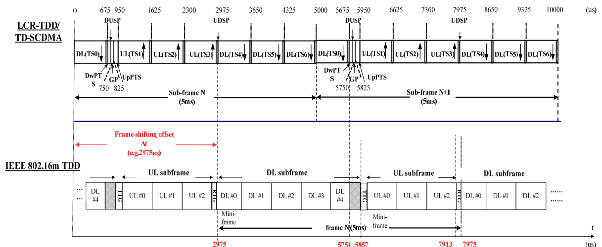
Figure 5: Radio frame coexistence structure of TD-SCDMA and IEEE 802.16m TDD
