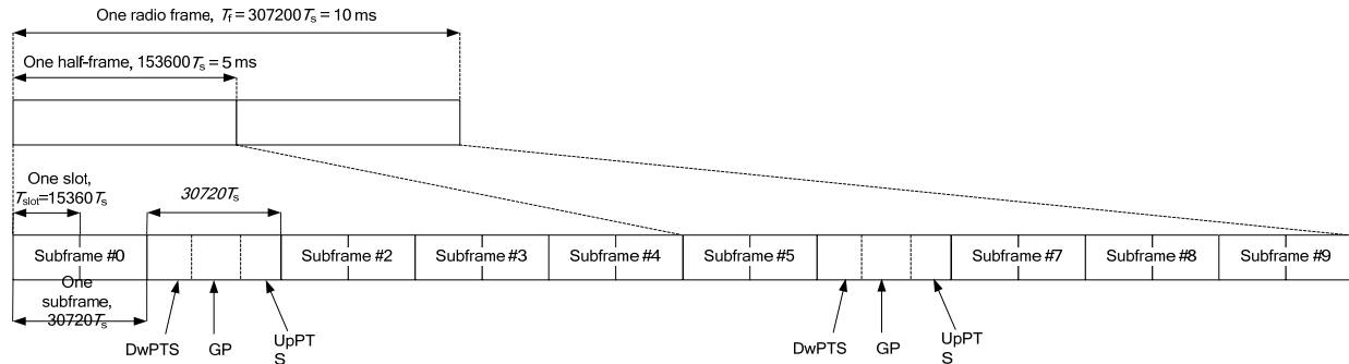
Figure 6 TDD LTE Radio frame structure of TDD mode in TS36.211
