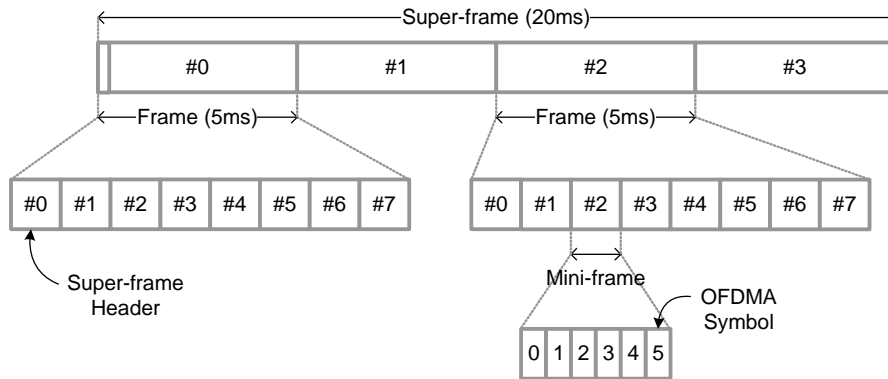
Figure 3 the Generic Frame structure assumed in IEEE 802.16m
