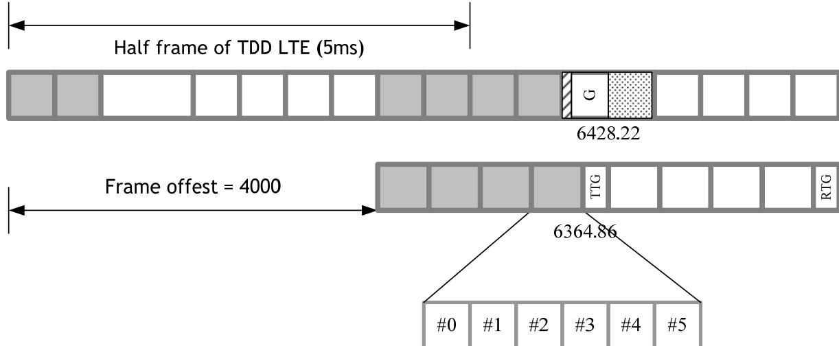
Figure 7 example of solution result when ratio of UL:DL = 1:1 for both IEEE 802.16m and TDD LTE
