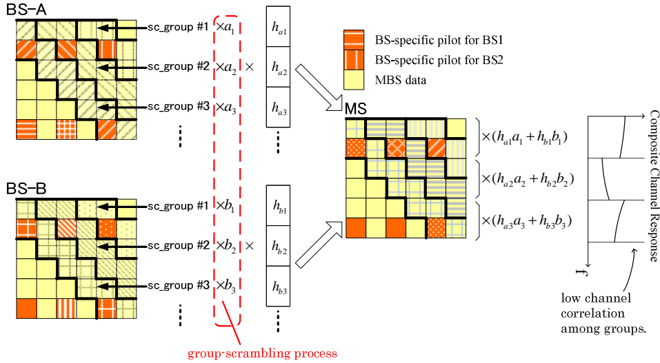
Fig.4 Proposed MBS structure with group-wised structure
