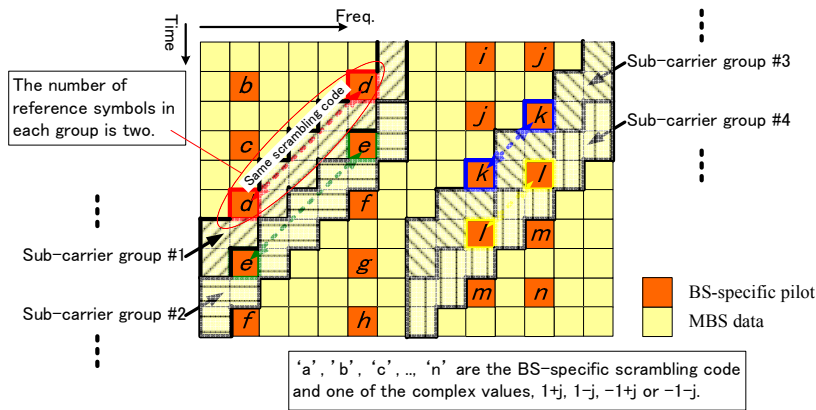
Fig.2 Sub-carrier group partition
