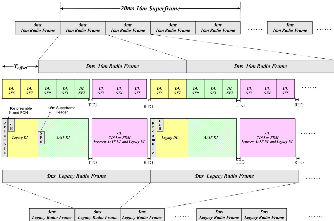
Figure 15.3.4.3-3 – Two switching point frame structure for supporting Legacy and AAIF
