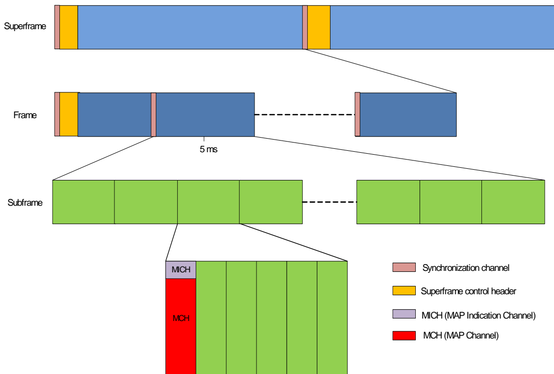
Figure xxx Example of DL control channel mapping
