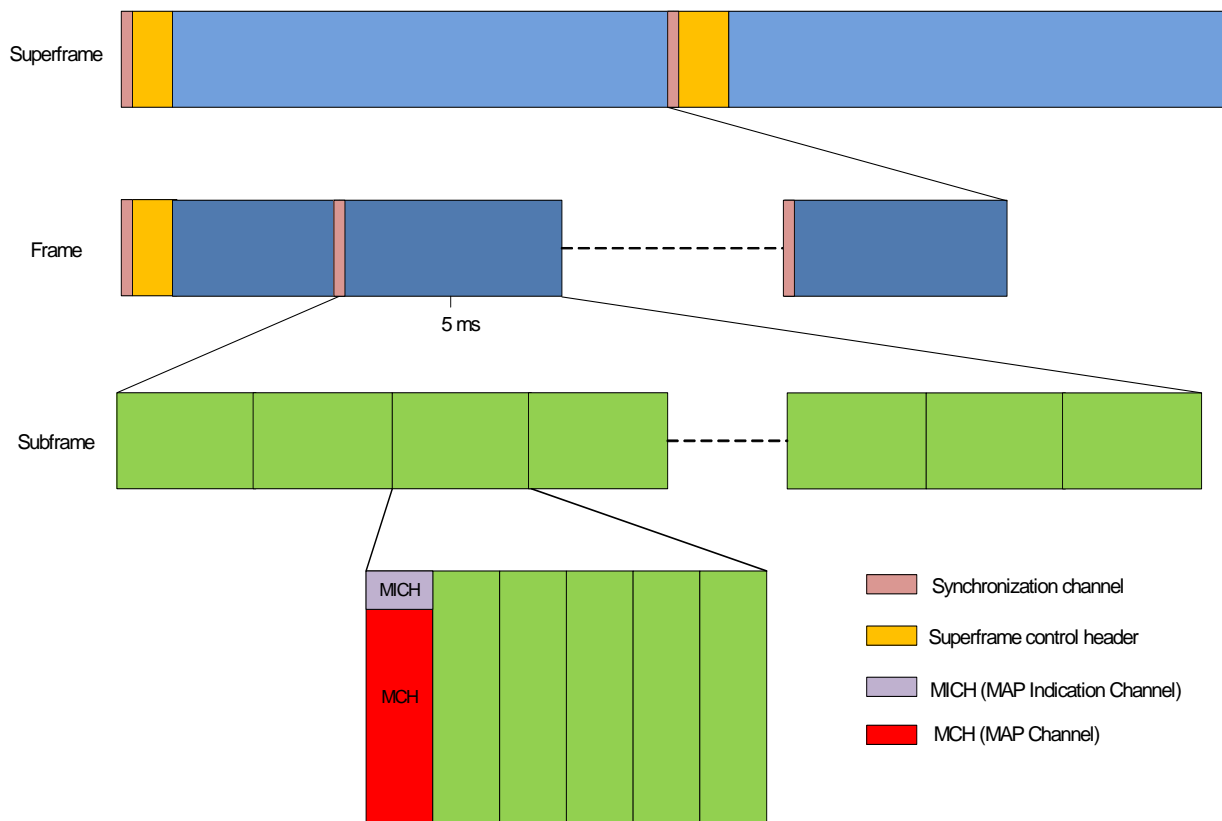
Figure 2 Proposed example of DL control channel mapping
