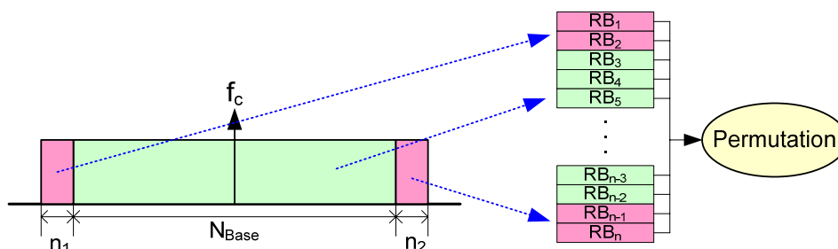
Figure xx1. Permutation using subcarriers including guard band subcarriers
