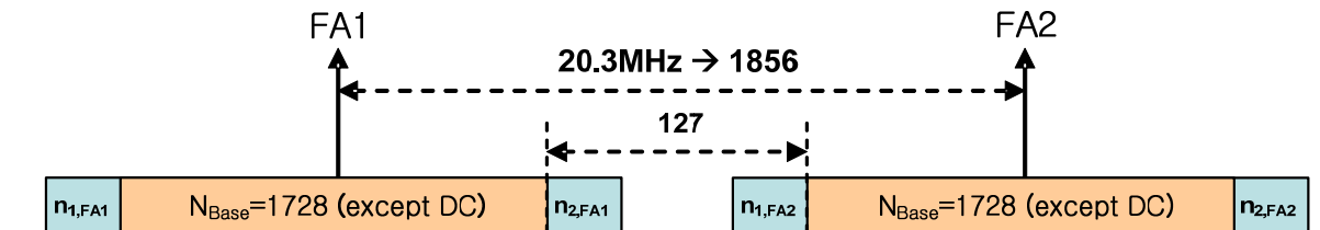
Figure 4. Using additional subcarriers in guard band (2048 FFT)
