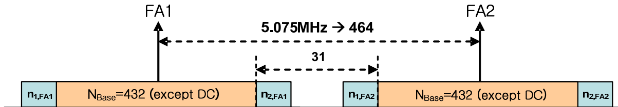
Figure 3. Using additional subcarriers in guard band (512 FFT)
