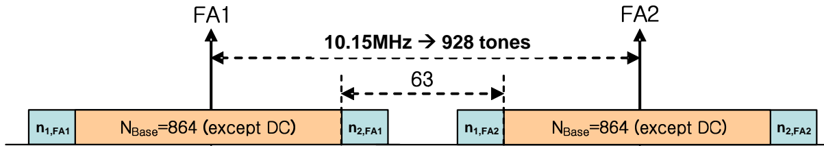
Figure 2. Using additional subcarriers in guard band (1024 FFT)
