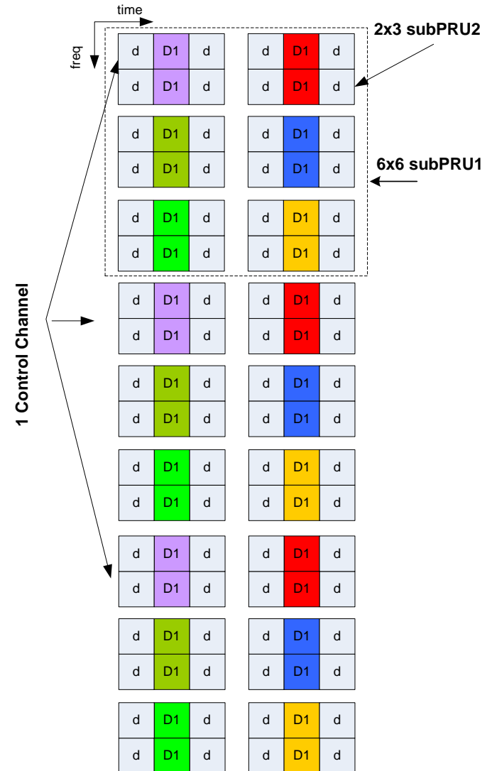
Figure 7: UL subPRU2 for control channel, SISO case
