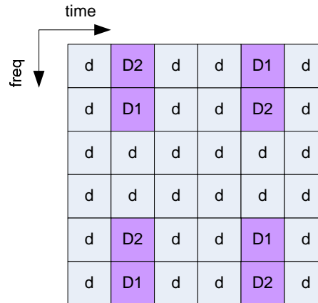
Figure 2: UL subPRU1, single user MIMO case
