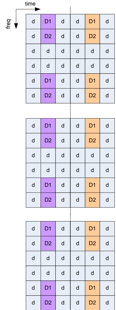
Figure 6: Special transmission for 48 data symbols, MIMO case
