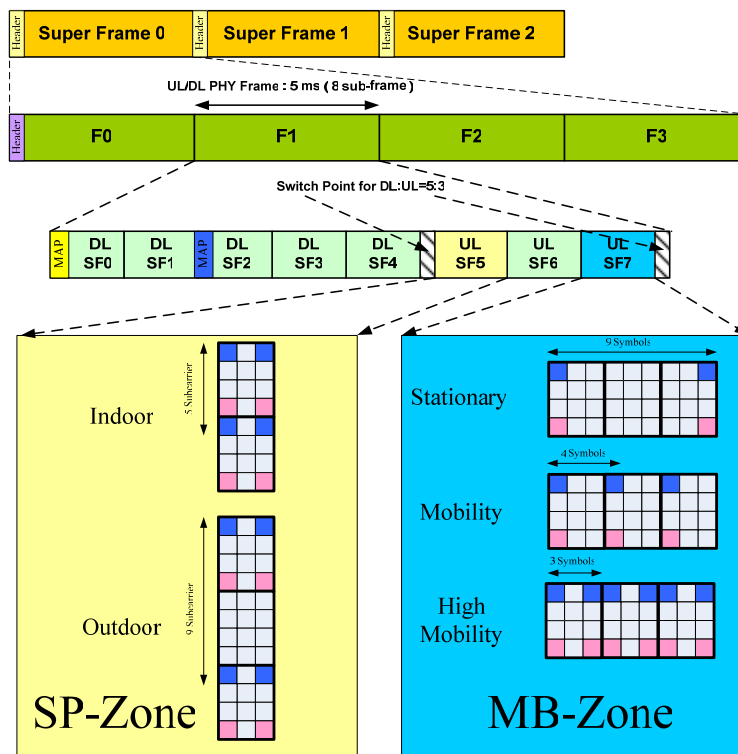
Fig.d Design example for the UL pilot structure by using SP-Zone and MB-Zone
