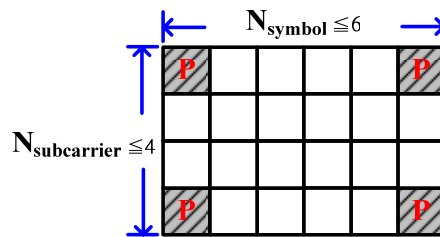
Fig. 1 The allocation of pilots
