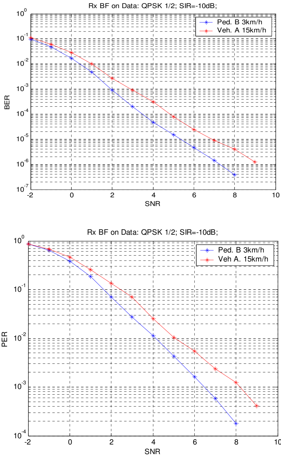
Fig. 9: Rx BF on Data: Mobility effect, Pedestrian B 3km/h.
