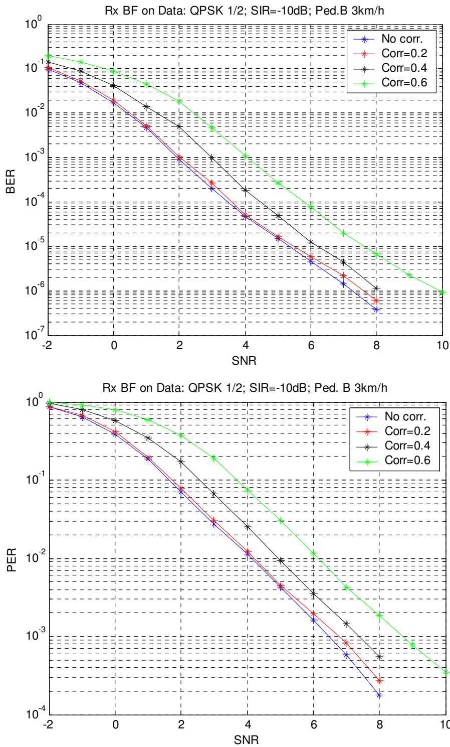
Fig. 10: Channel Correlation effect; SIR=-10dB, Pedestrian B 3km/h.
