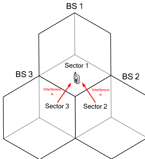
Fig.3 Neighboring BSs Sectors are the Interfering Sources
