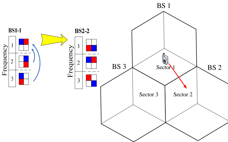
Fig.X.1 An MS Moves from BS1-1 to BS2-2 it Selects and Changes its Pilot Pattern Orthogonal to the Pilot Pattern of BS2-2
