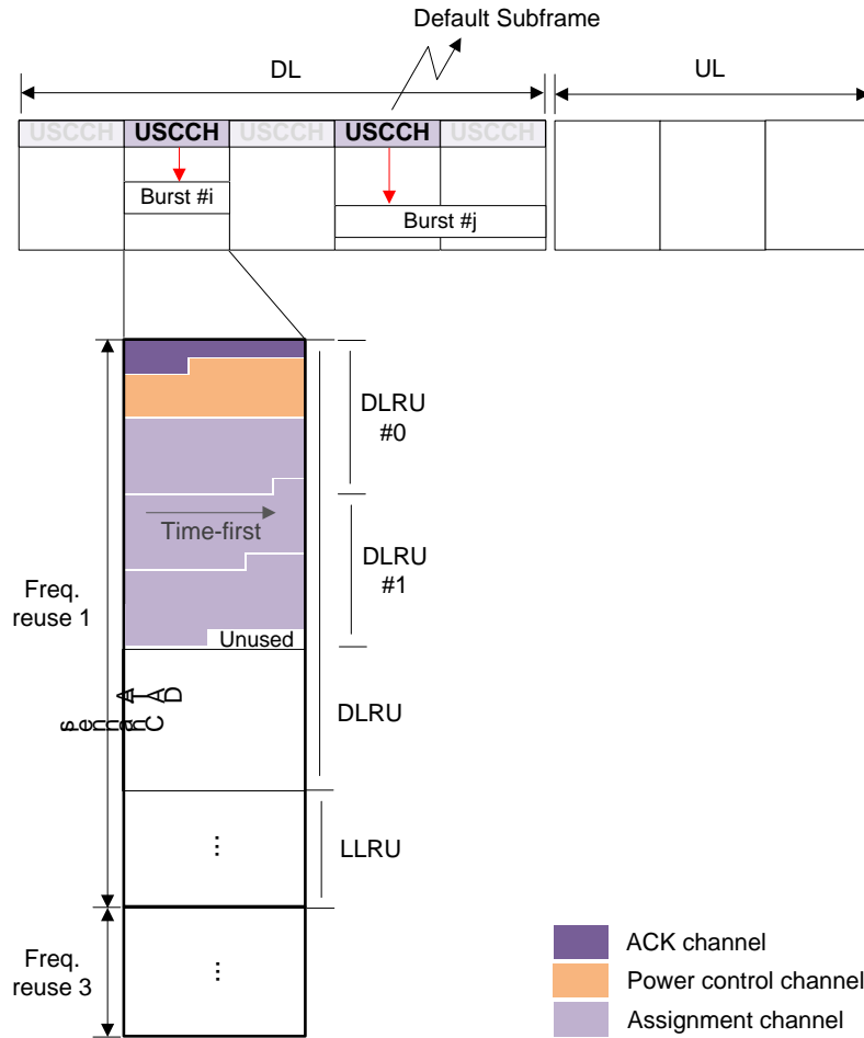
Figure 1 – Logical USCCH structure
