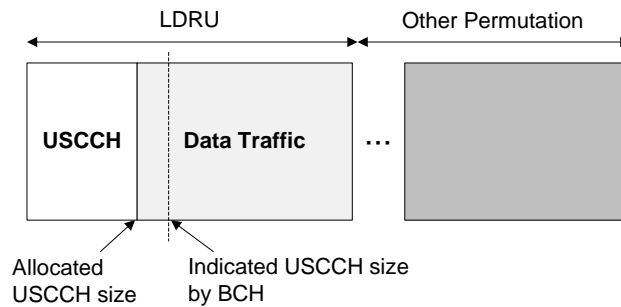
Figure 2 – Signaling of USCCH size
