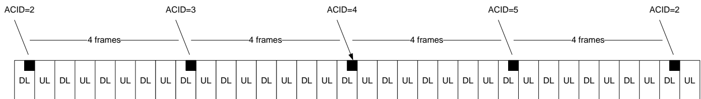
Figure 7 – An example of HARQ channel identifier
