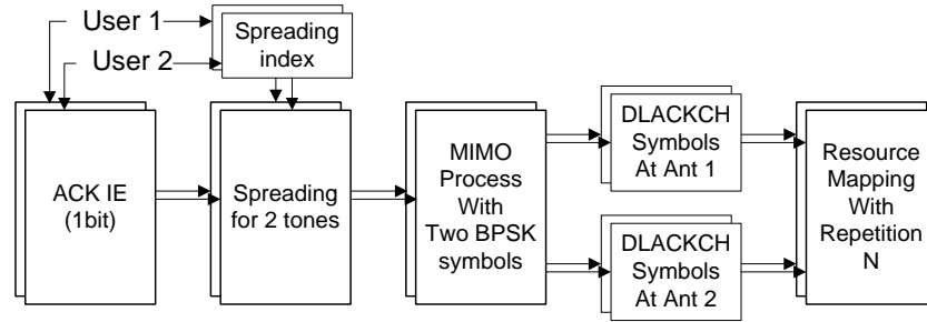
Figure 4 – Block diagram of DLACKCH symbol generator
