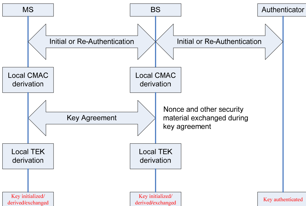
Figure 1 Initial or Re-authentication - Key Derivation and Exchange
