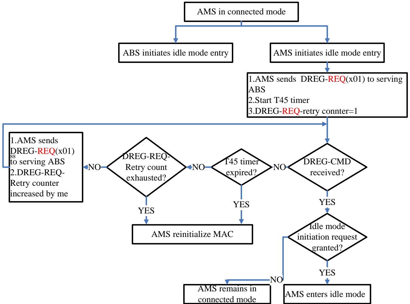
Figure 417—Procedures during AMS initiates idle mode entry
