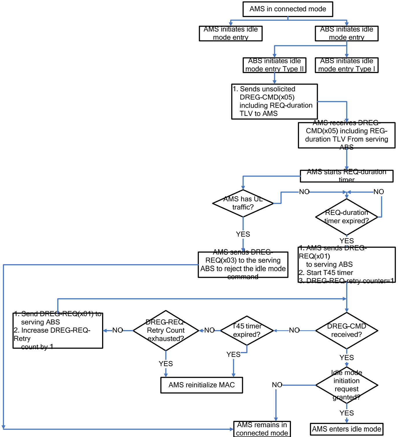
Figure 420–Procedures during Type 2 ABS initiates idle mode entry
