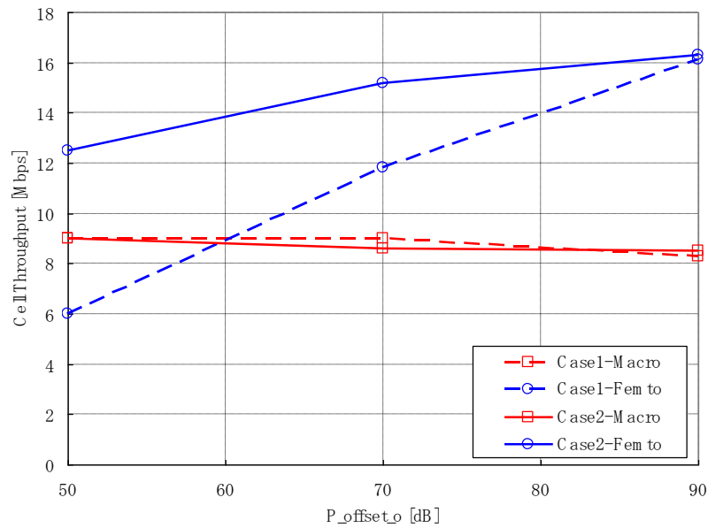
Fig.2 Dependence of Cell Throughput on P_offset_o
