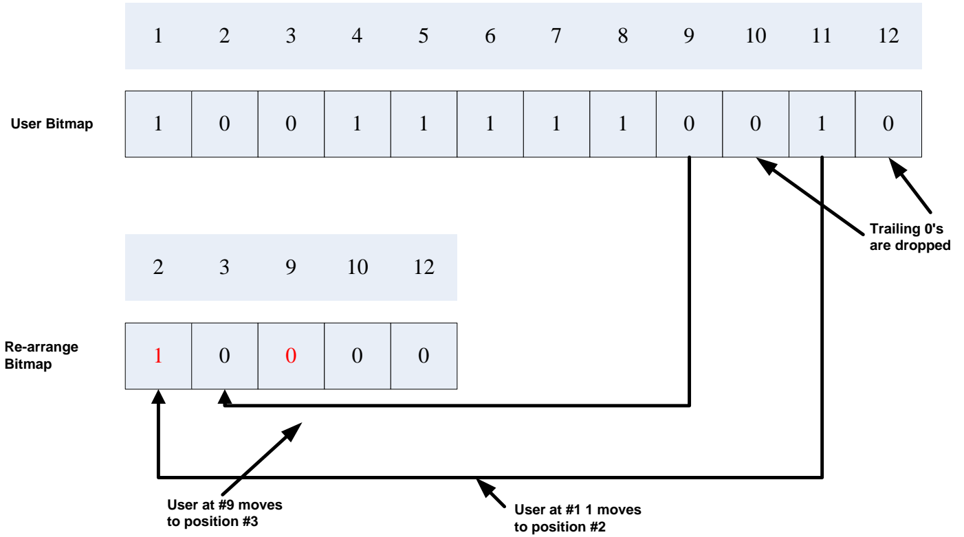
Figure 420-Example of re-arrange user bitmap
