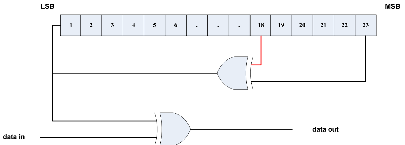
Figure 492- The Data randomization with a PRBS generator (1+x^{18}+x^{23})
