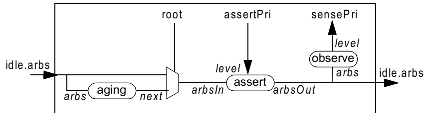
Figure 20—Arbitration controls
