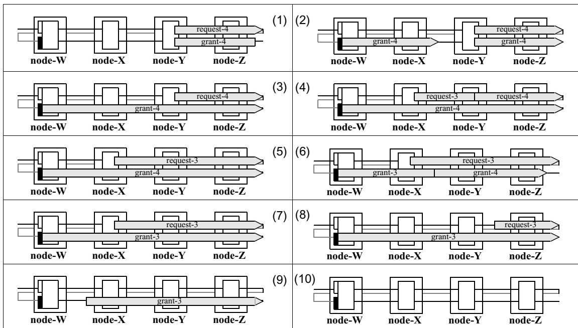
Figure 9—Prioritized arbitration
