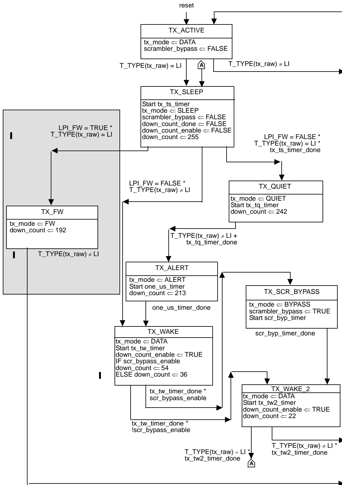
Figure 82-1—LPI Transmit state diagram
