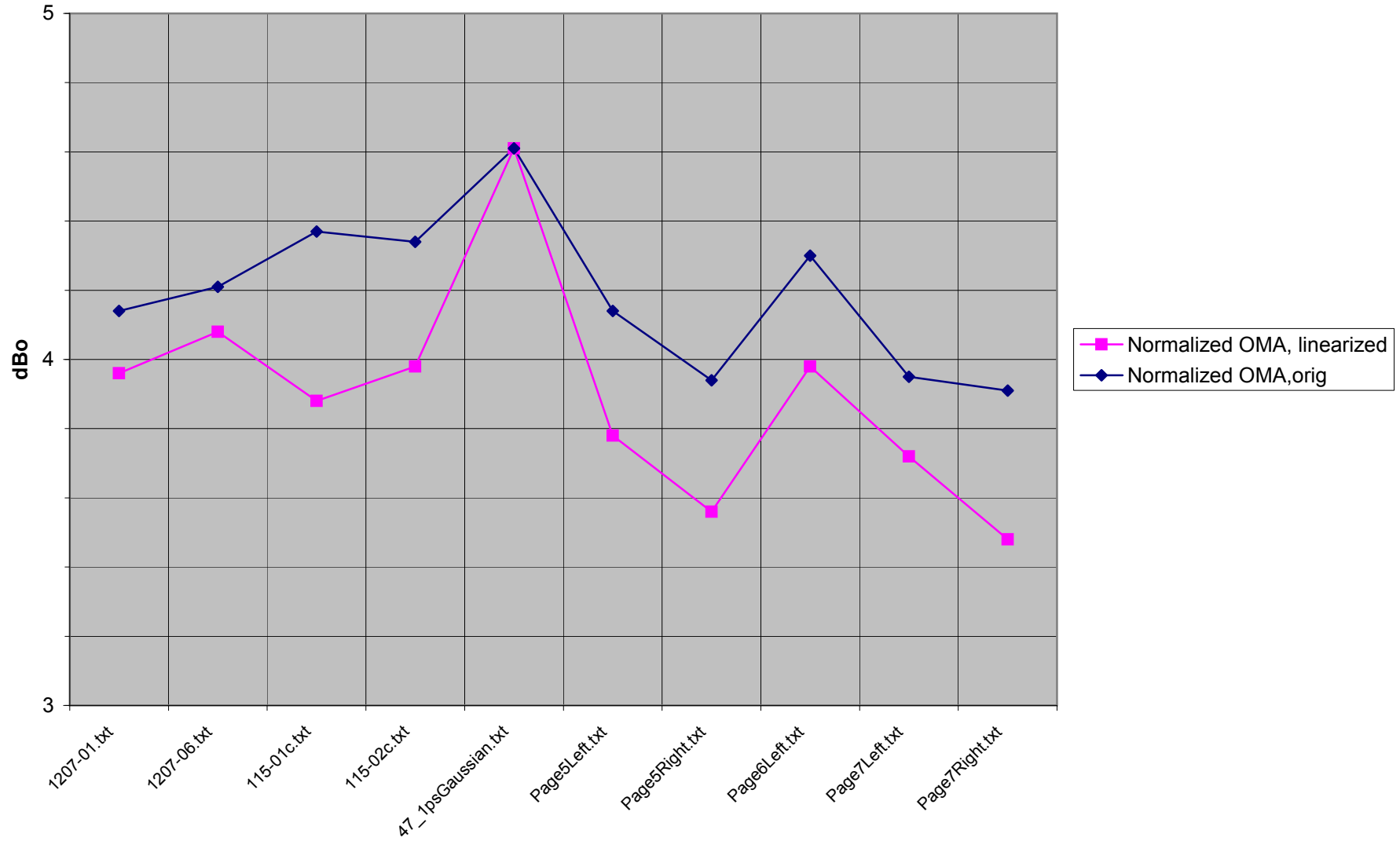
Orig vs. Linearized Waveform, TWDP (FF=100, FB=50)
