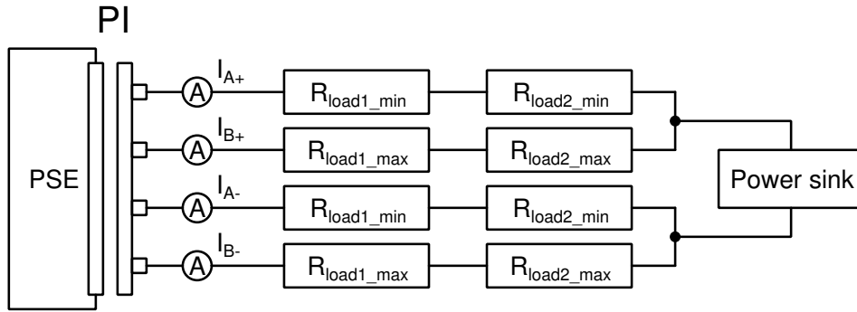
Figure 145–22 — PSE current unbalance verification circuit
