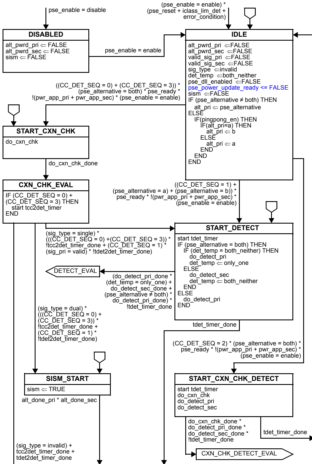
Figure 145–13—Top level PSE state diagram
