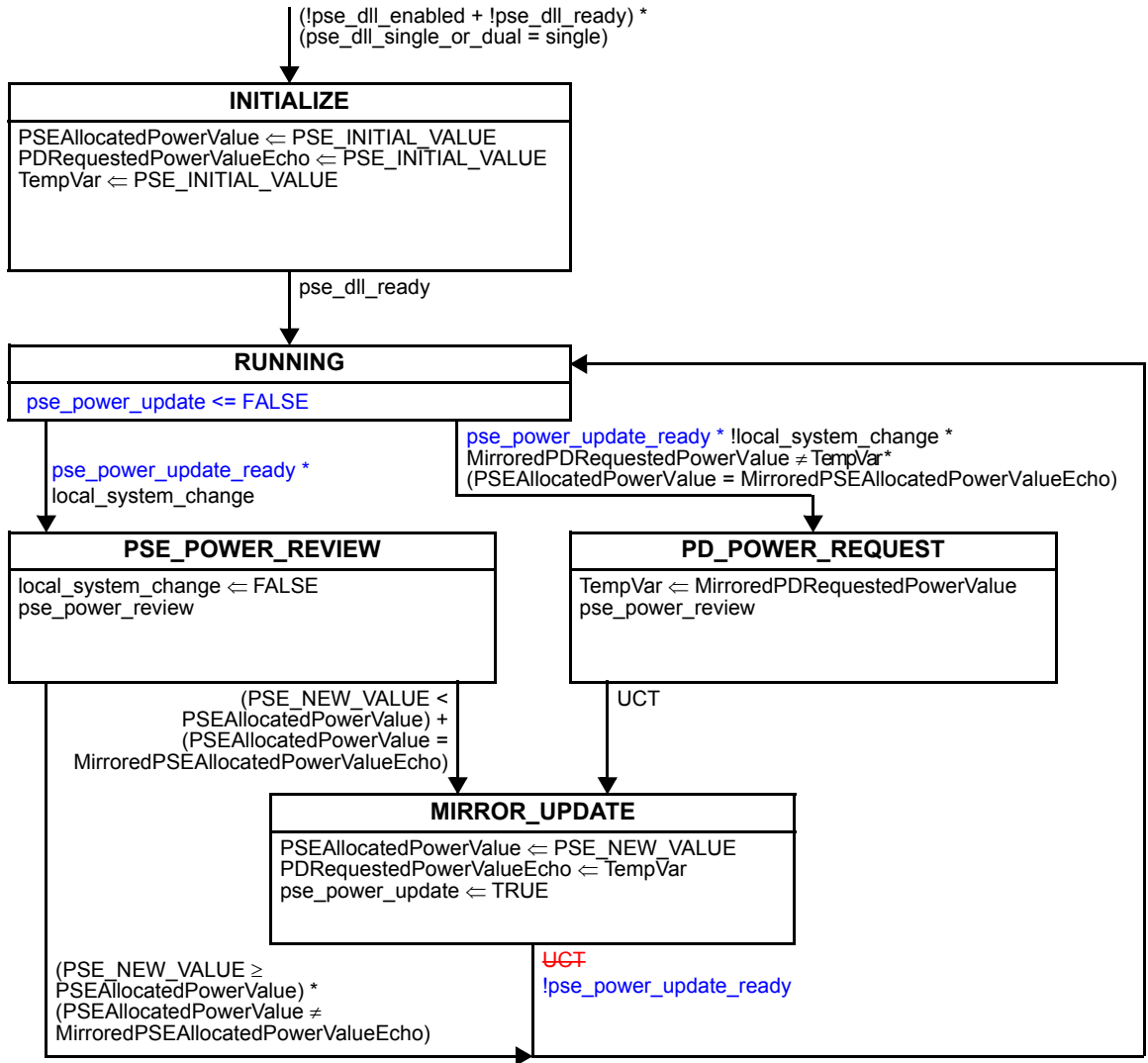
Figure 145-43—PSE power control state diagram
