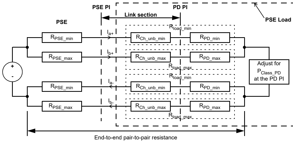
Figure 0-1—PSE PI unbalance specification and system resistance unbalance
