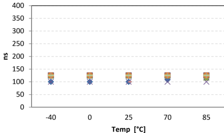
Shutdown Time to Powersaving
