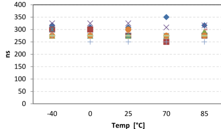
Startup Time from Powersaving
