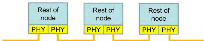
Linear Switched Topology
