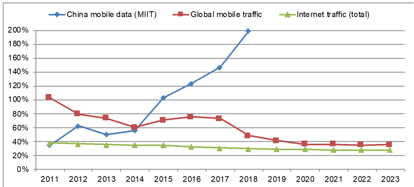
Figure 27- Comparison of Growth Rates [17]
