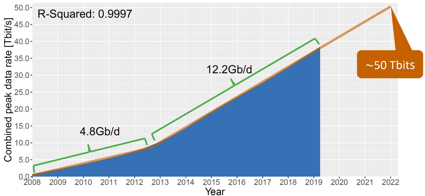
Figure 39- Euro-IX IXP Peak Data Rate Trend [19]
