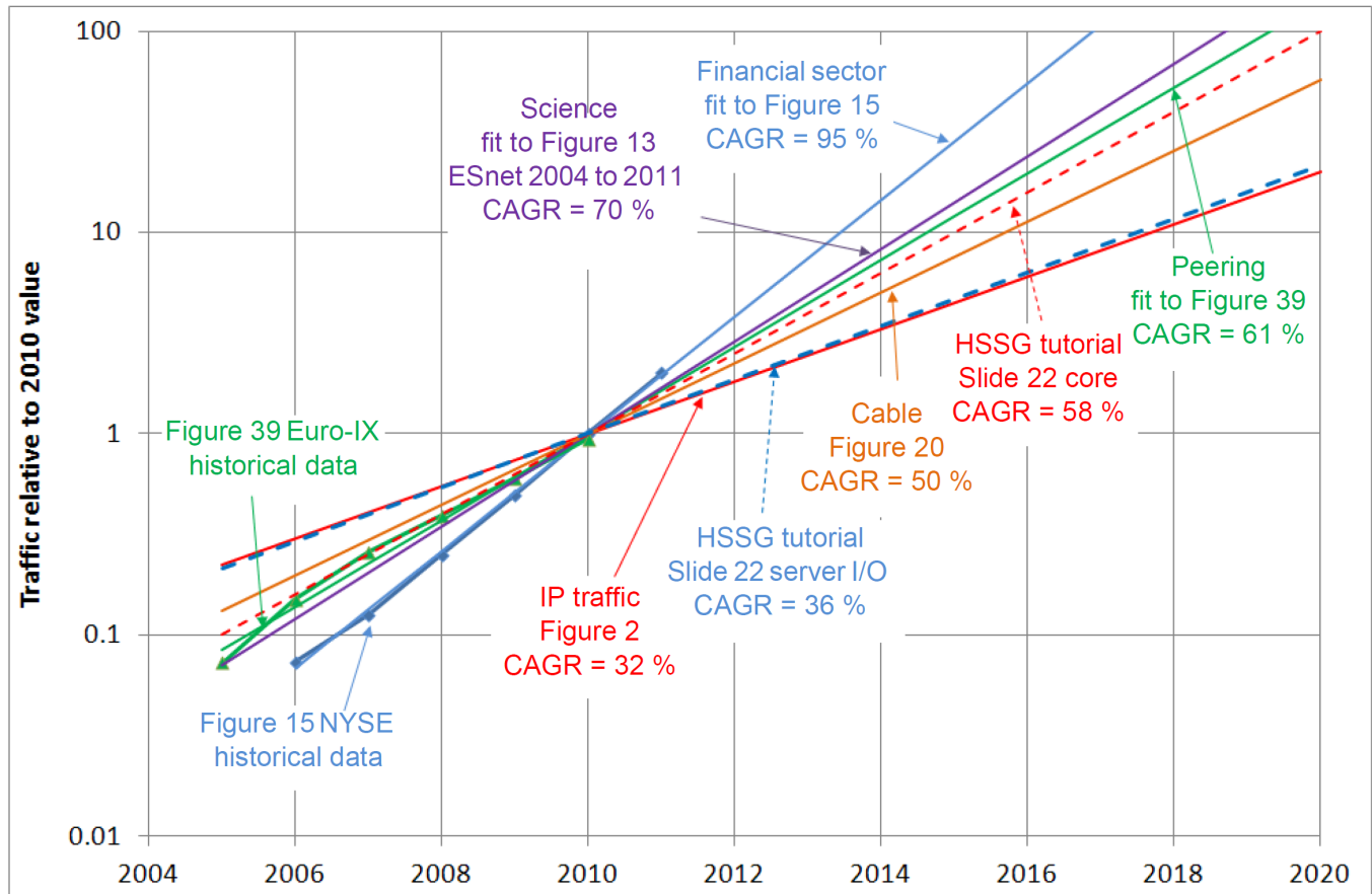
Figure 47- 2012 IEEE 802.3 Ethernet Bandwidth Assessment Forecast [1]
