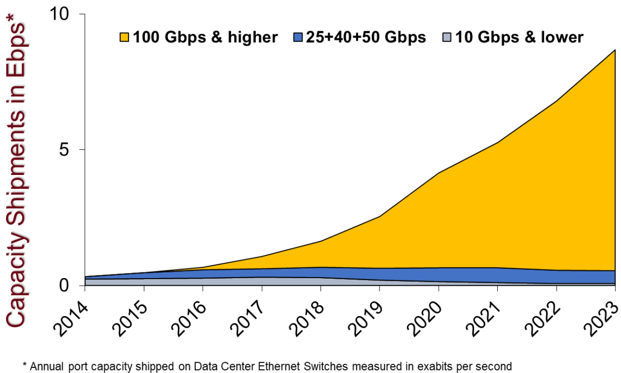
Figure 29- Data Center Ethernet Switch Capacity Shipments [21]
