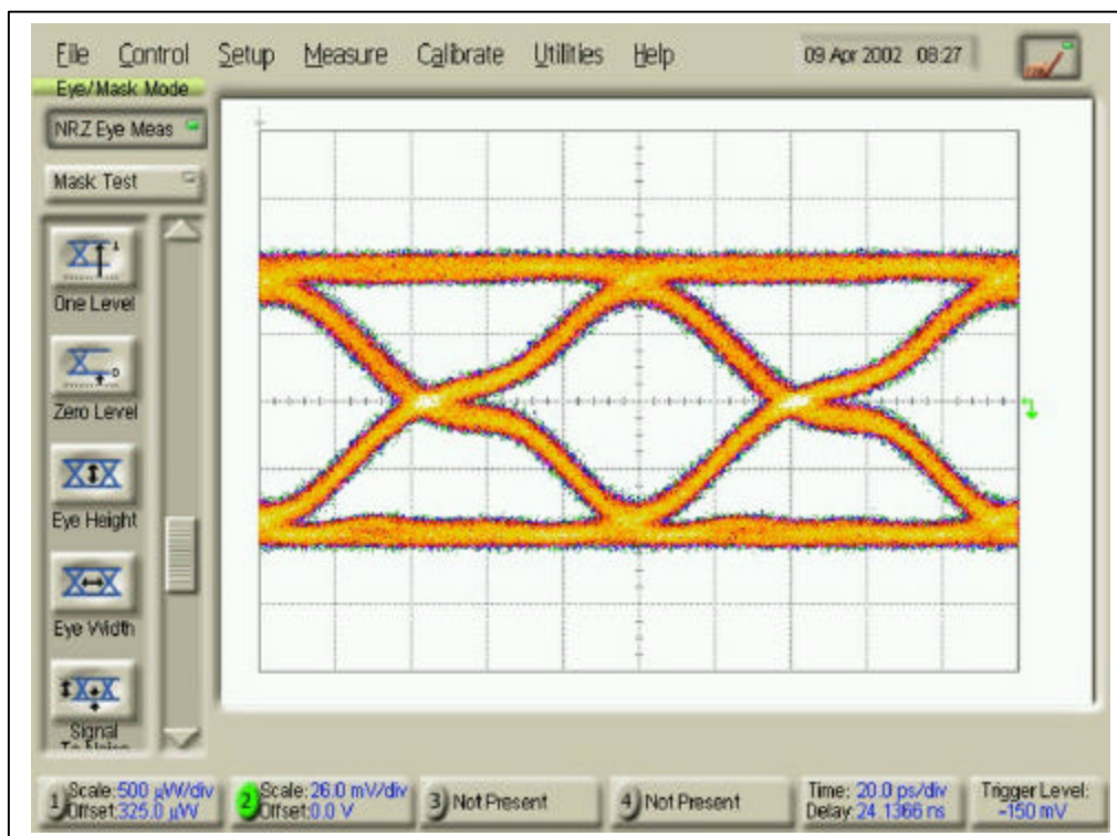
Eye pattern for 10.3125G-b/s NRZ signal at 2^{31}-1 PRBS through transversal filter
