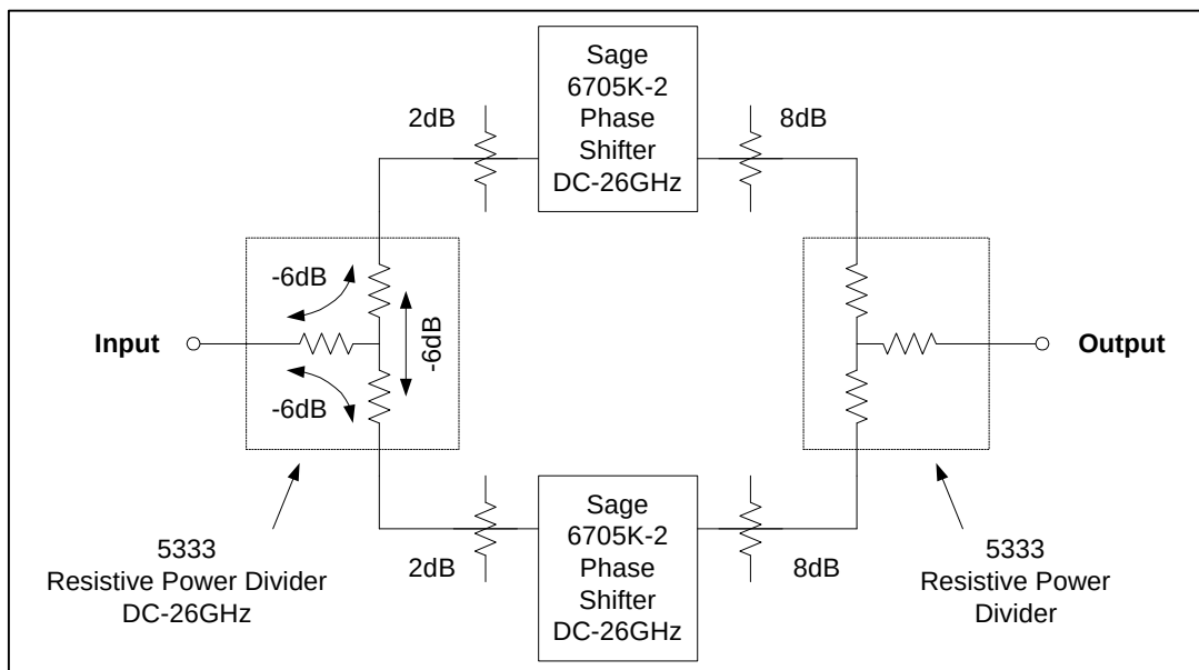
Test setup with phase shifters set for a null in S_{21} at 8.945 GHz
