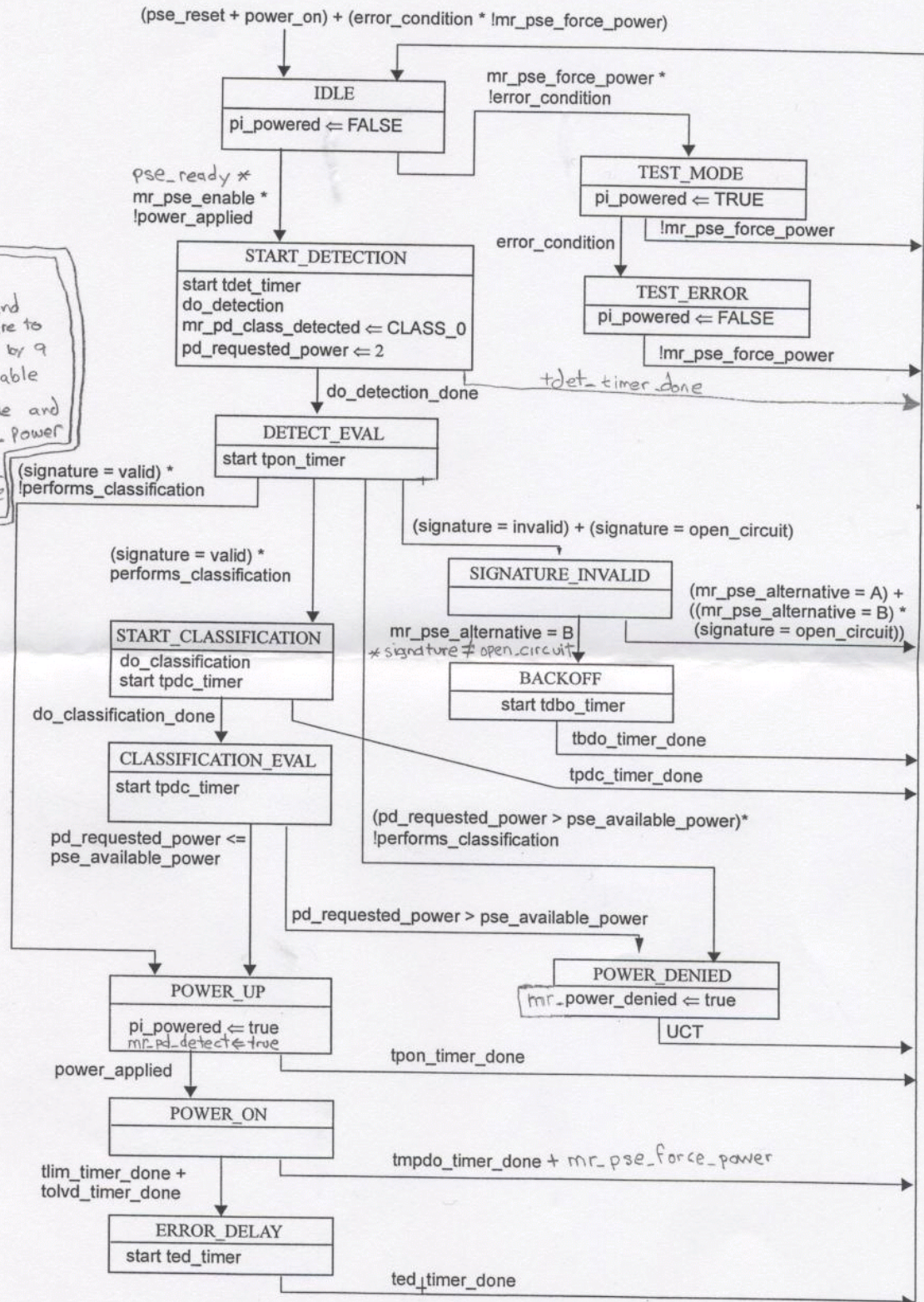
Figure 33-5—PSE state diagram
