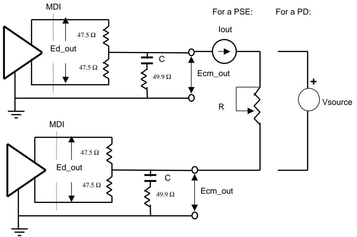
Figure 33-35—PSE and PD termination
