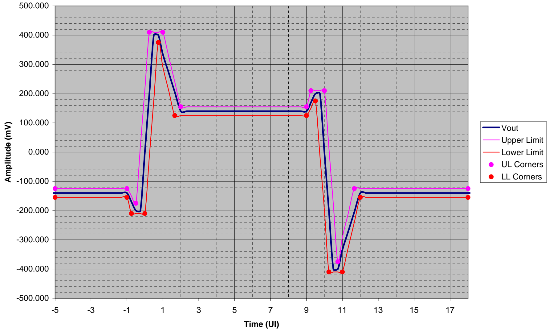
Transmitter Output Waveform
