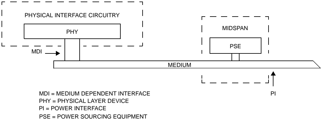
Figure 33-3a—DTE Power via MDI midspan power sourcing equipment relationship to the physical interface circuitry and the IEEE 802.3 CSMA/CD LAN model
