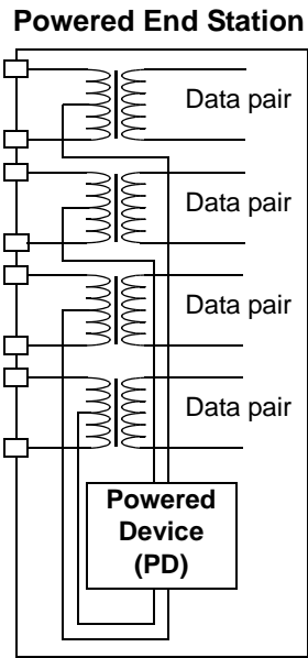
Figure 33-4A—100BASE-T PSE
