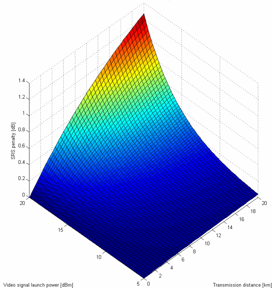
SRS penalty for minimum fibre attenuation @ 1550 nm [+5dBm]
