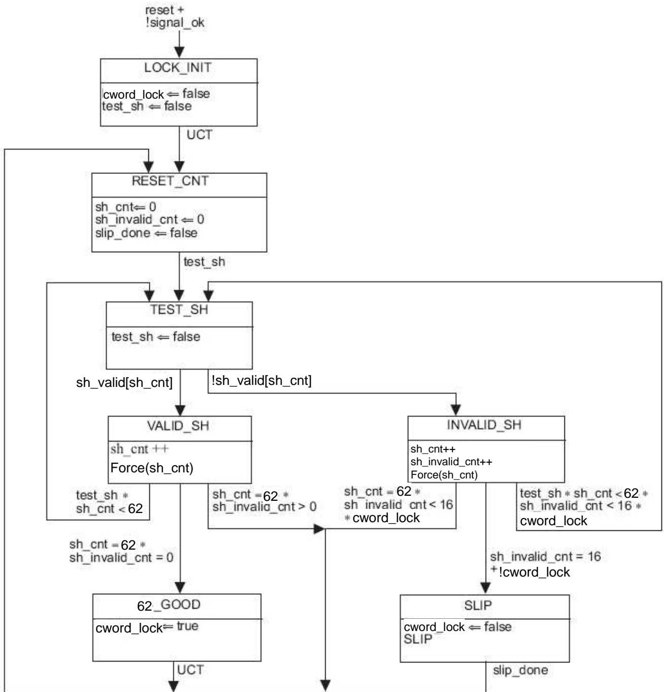
Figure 49-12—Lock state machine
