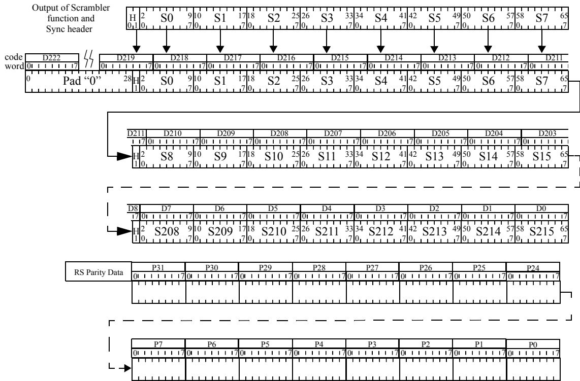
Figure 92-1—Bit ordering in FEC codeword generation
