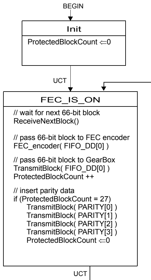
Figure 1-1—OLT Data Detector state machine
